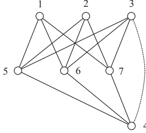
Figure 4: 2-adjacent Kuratowski subgraphs H_1 and H_2 .
