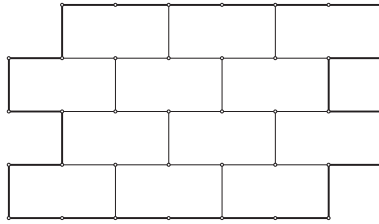
Figure 2: An (8 \times 5) -wall and its perimeter
